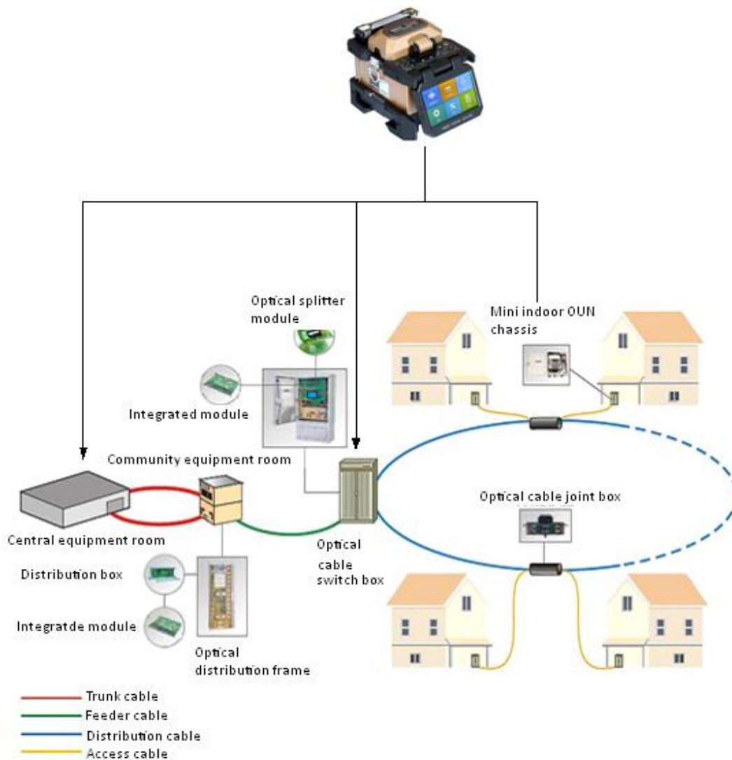
Typical application of AV6481B Optical Fiber Fusion Splicer
